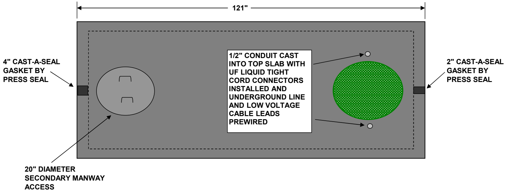
TOP VIEW
