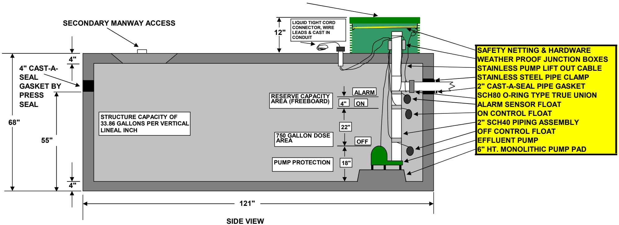
SIDE VIEW
