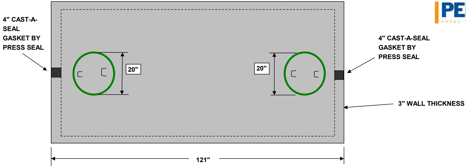
TOP VIEW
